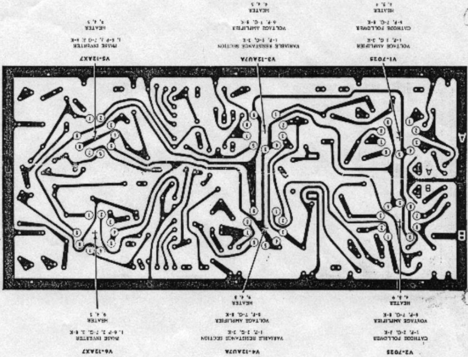
Fig. 70. PRINTED CIRCUIT BOARD - MODEL 534 DUAL CHANNEL AMPLIFIER (UNDER SIDE)
