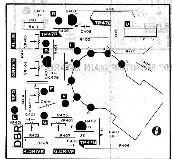
13" MONITOR NECKBOARD
