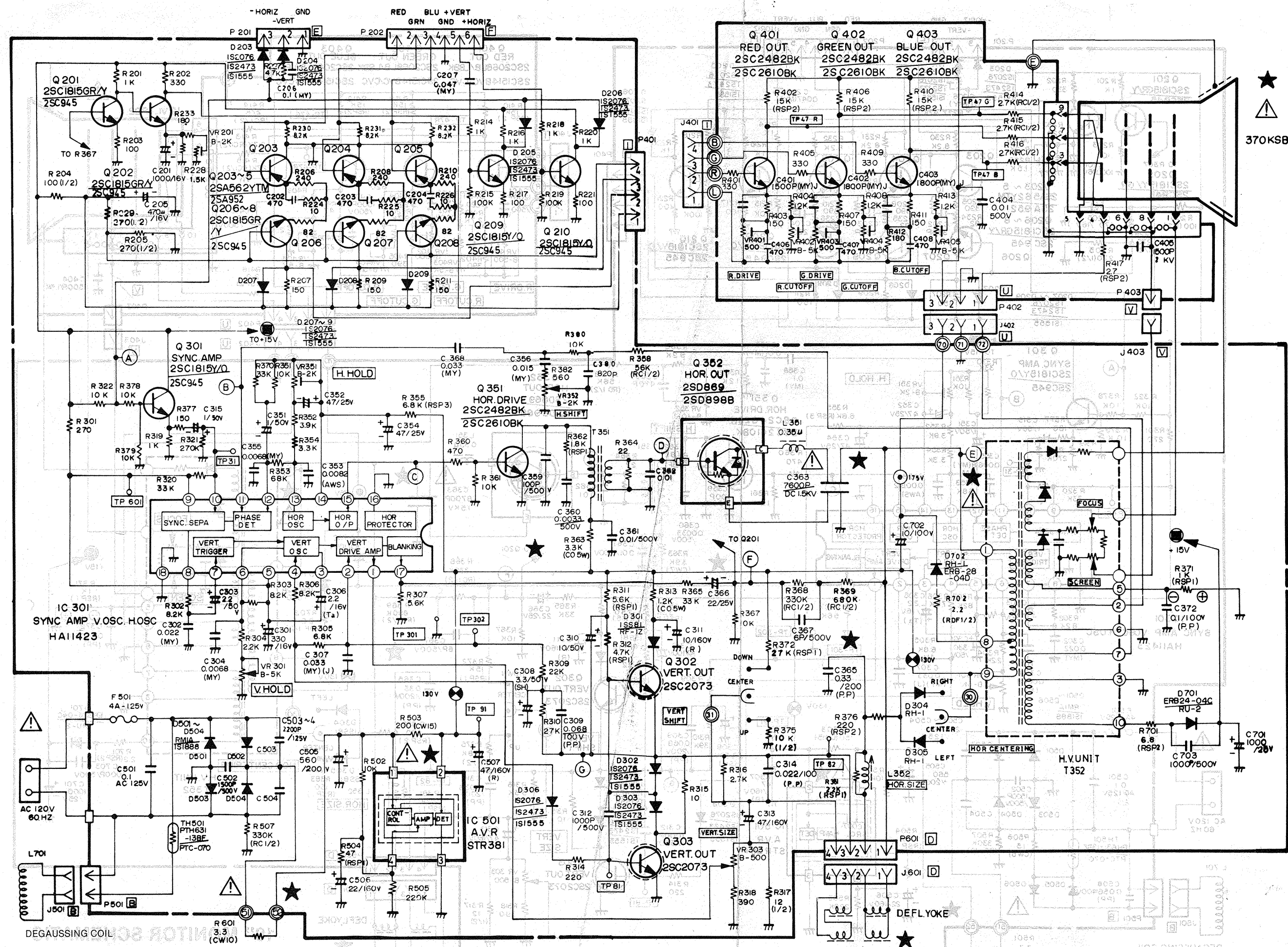
13" MONITOR SCHEMATIC
