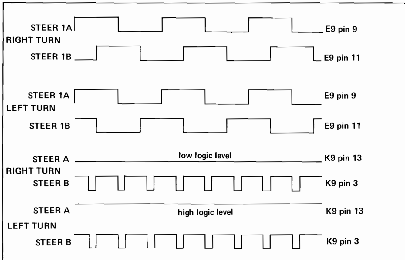
Figure 8-1 Steering Signals
