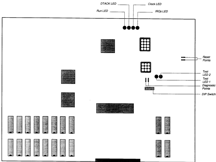
Figure 3-1 DIP Switch and LED Locations on the Multisync PCB
