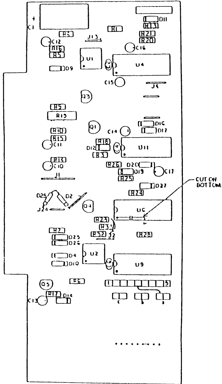
2X3781 COMPONENT LAYOUT
