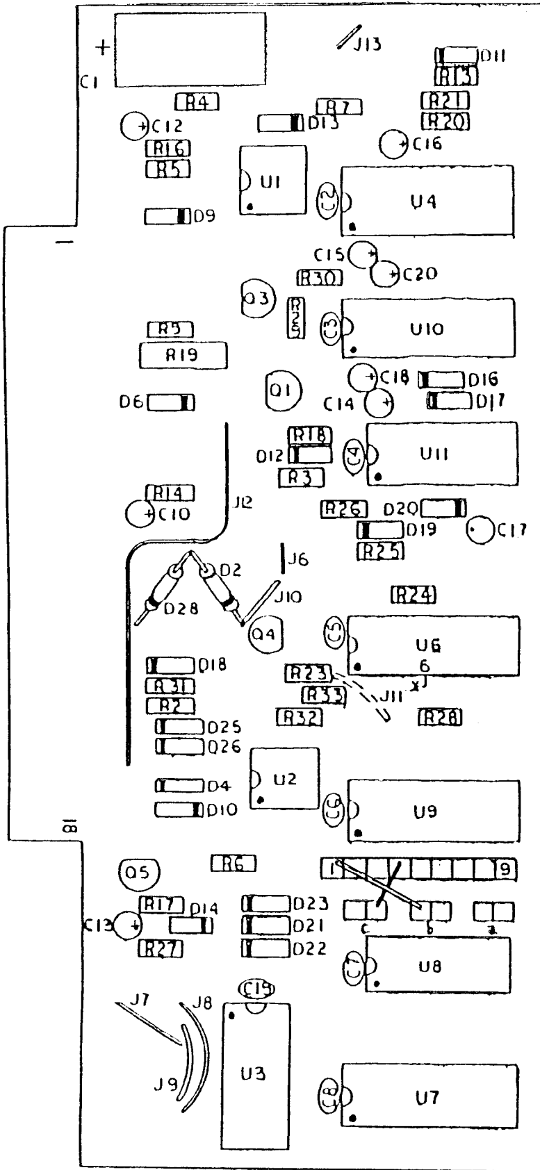
2X4016 COMPONENT LAYOUT
