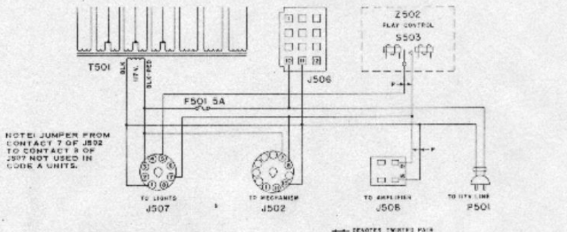
Type TSU2 Primary Circuit (Cont'd)
