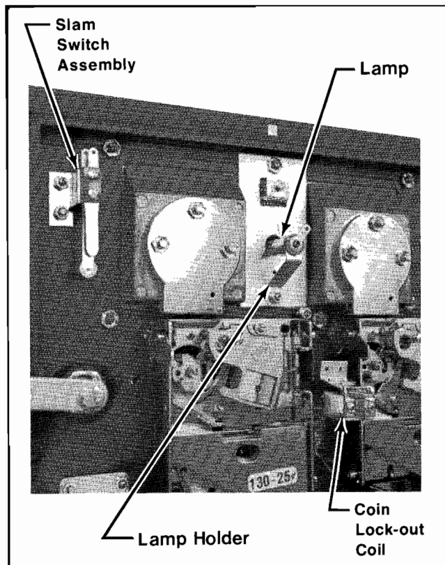
Figure 8 Coin Door Assembly
