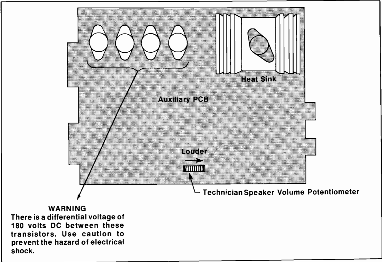
Figure 21 Location of Technician Adjustment for Speaker Volume
