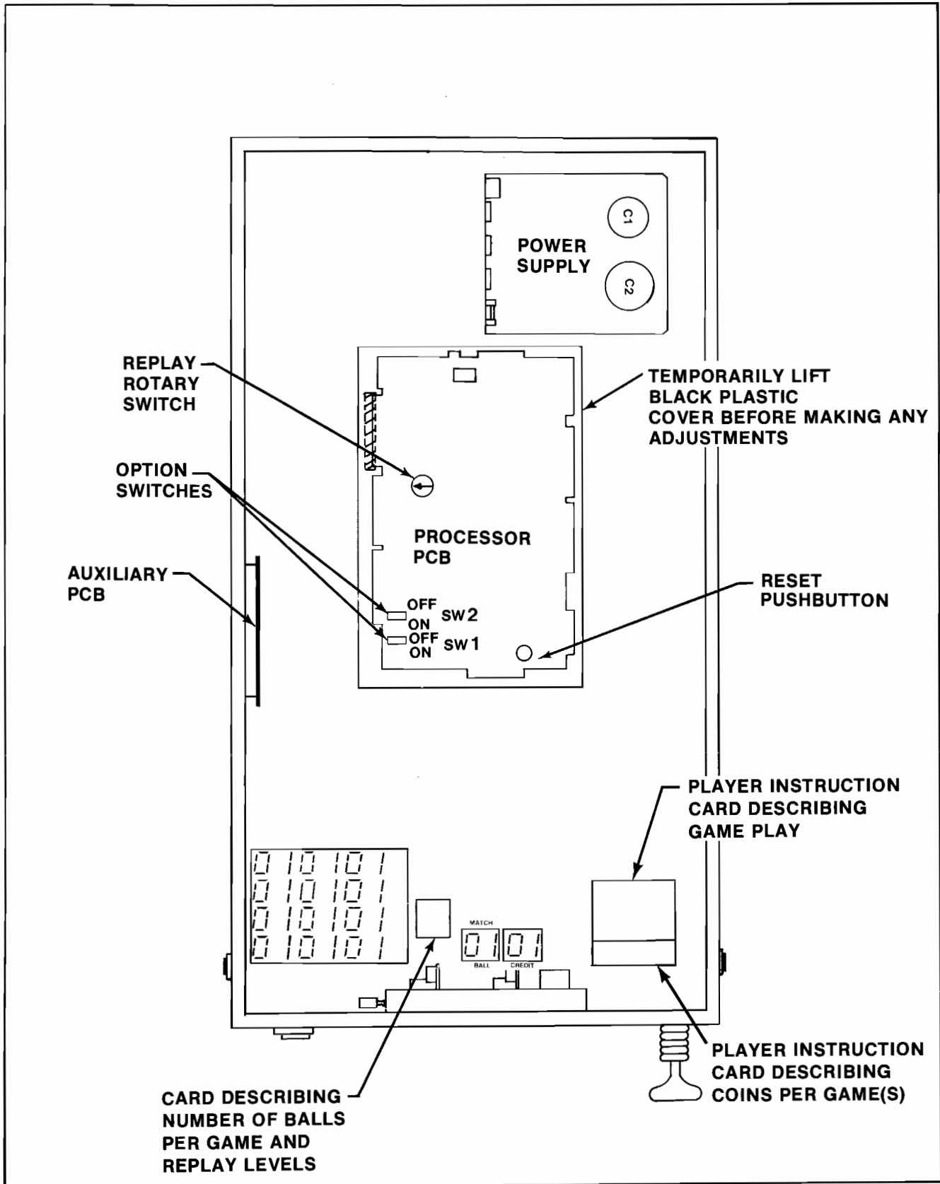
Figure 5 Location of Option Switches
