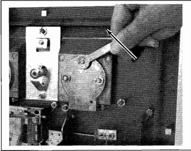
Figure 12 Removal of Plate Covering Rear of Coin Slot
