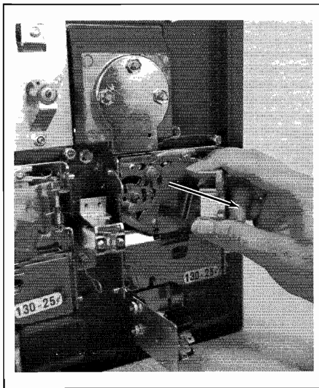
Figure 9 Hinging Open the Magnet Gate Assembly
