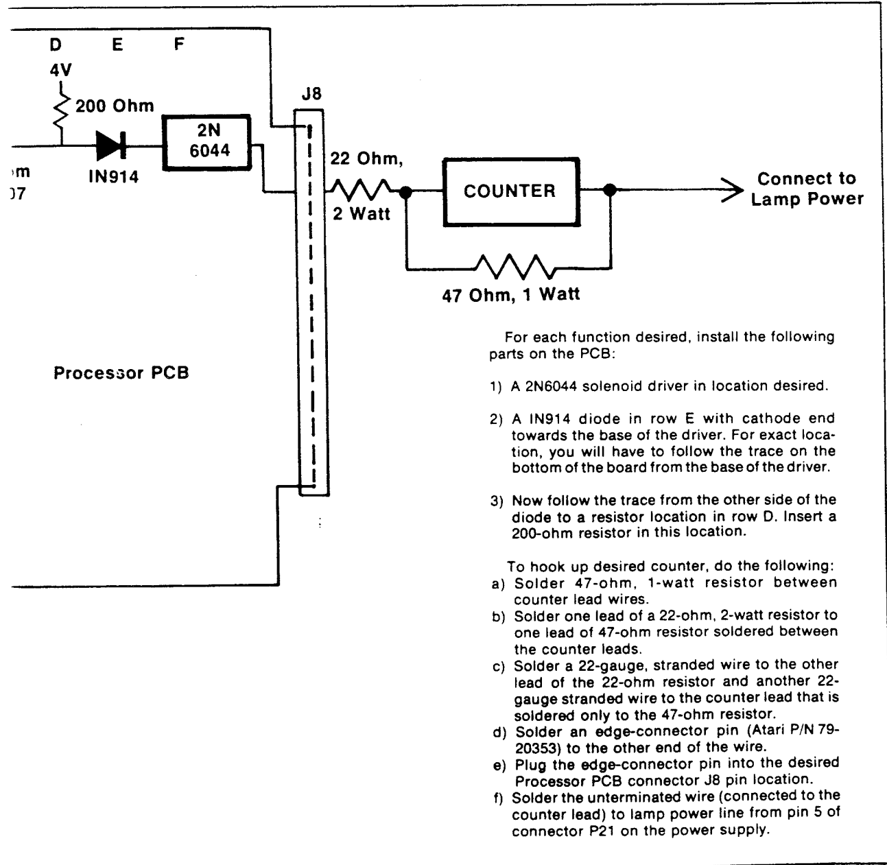
Figure 30 Additional Components to be Installed for Each Metering Function Added
