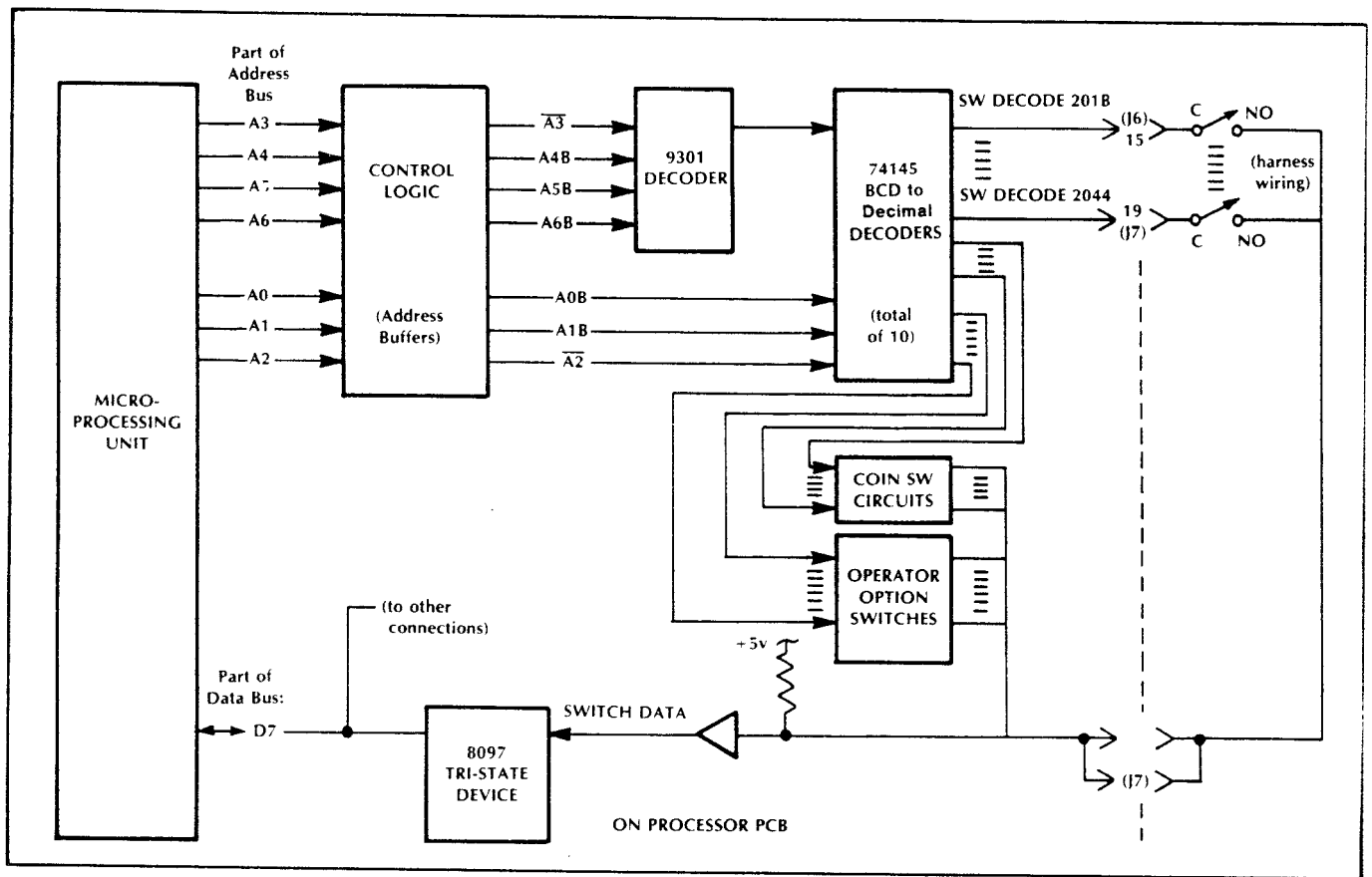
Figure 32 Simplified Diagram of Switch Sensing Circuit
