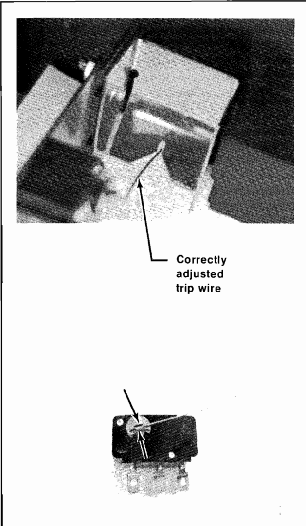
Figure 13 Detail View of Coin Switch and Trip Wire
