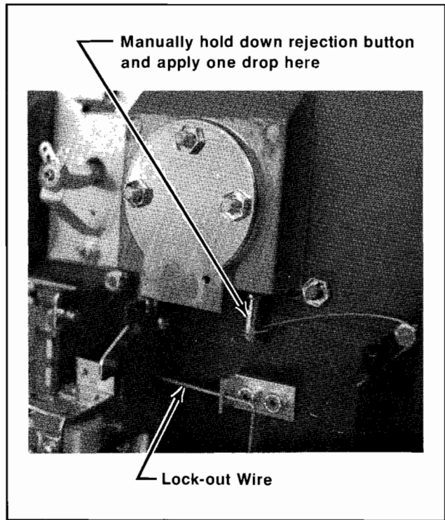
Figure 15 Close-up View of Lubrication Point
