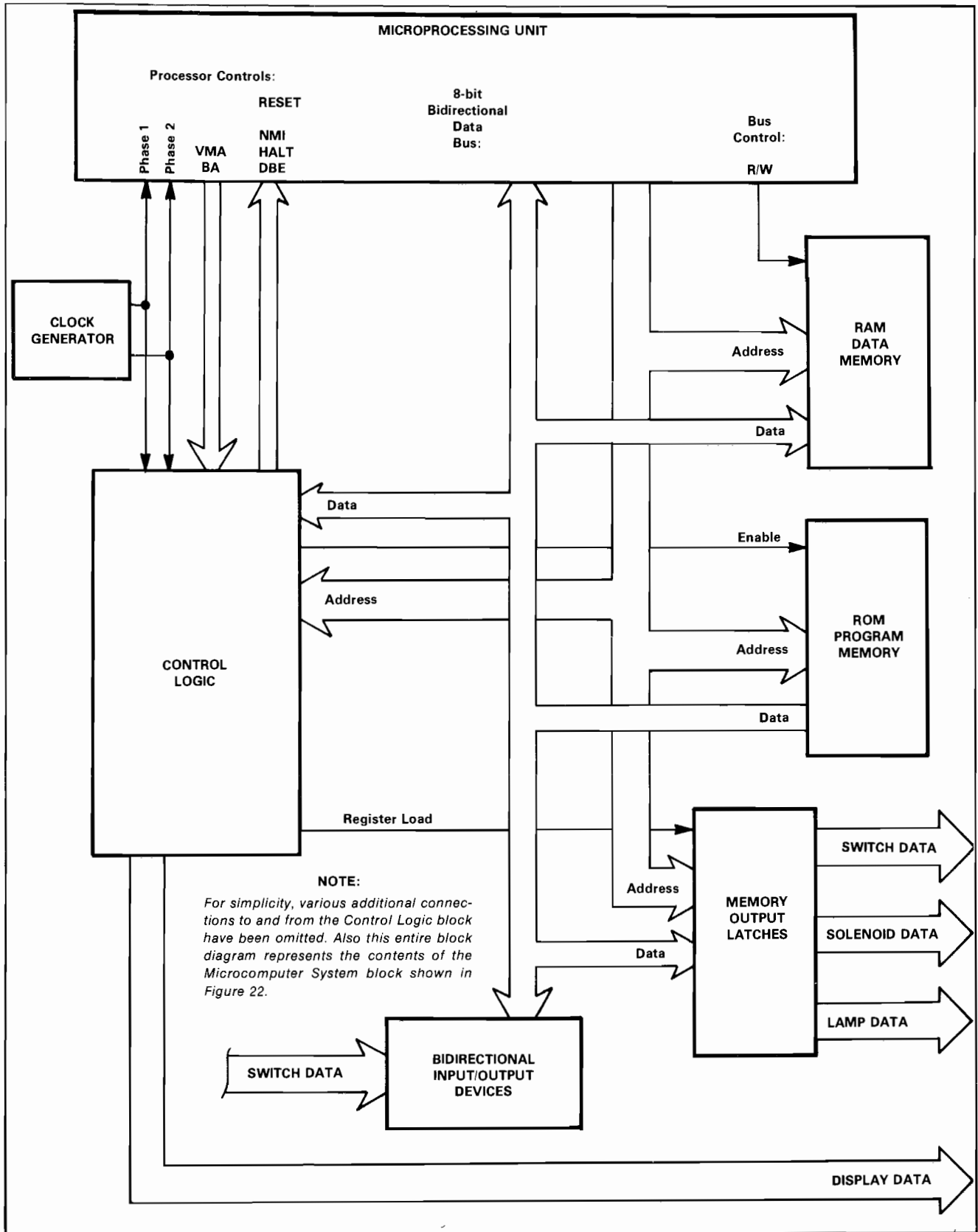
Figure 23 Block Diagram of Microcomputer System
