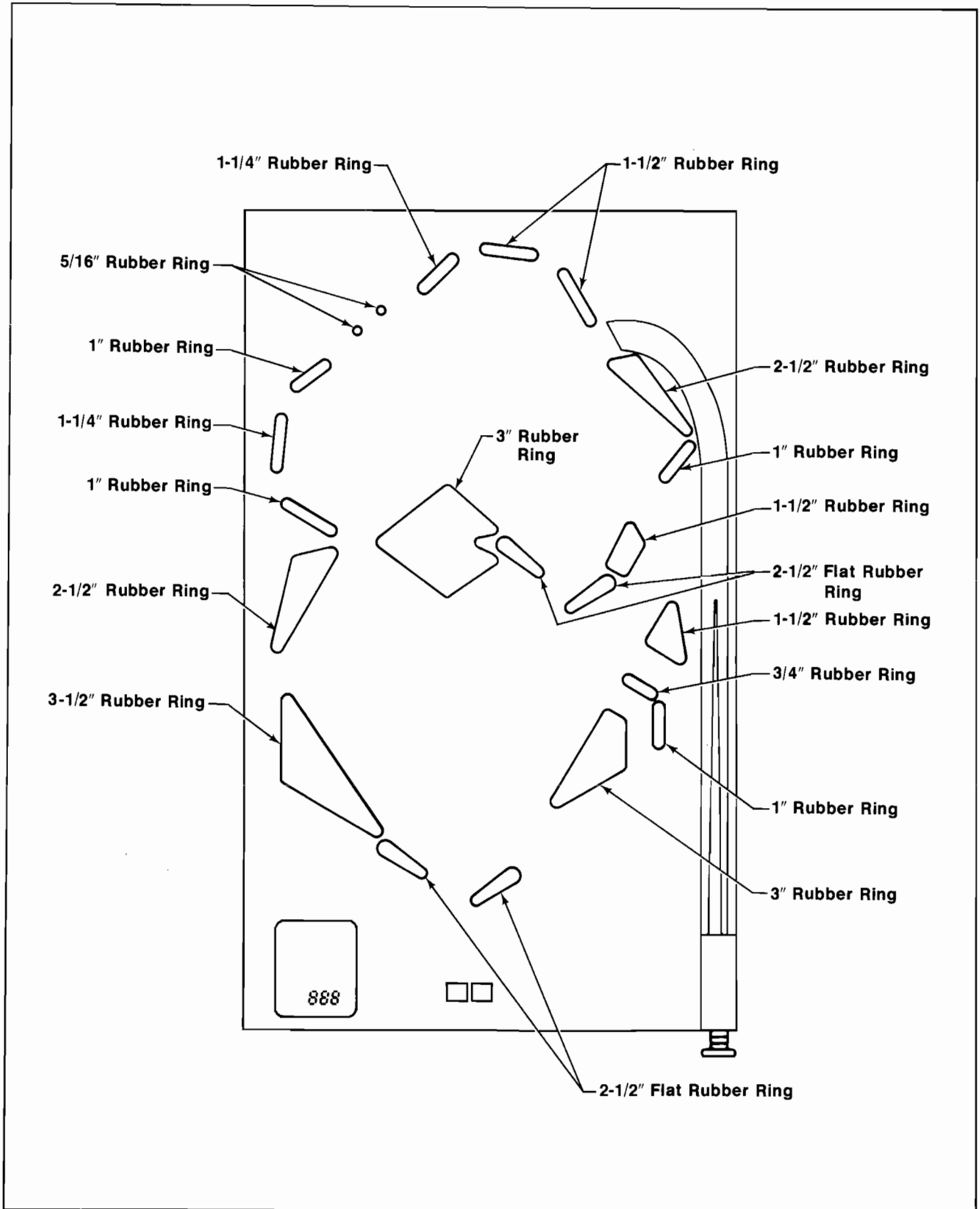
Figure 7 Playfield Rubber Sizes
