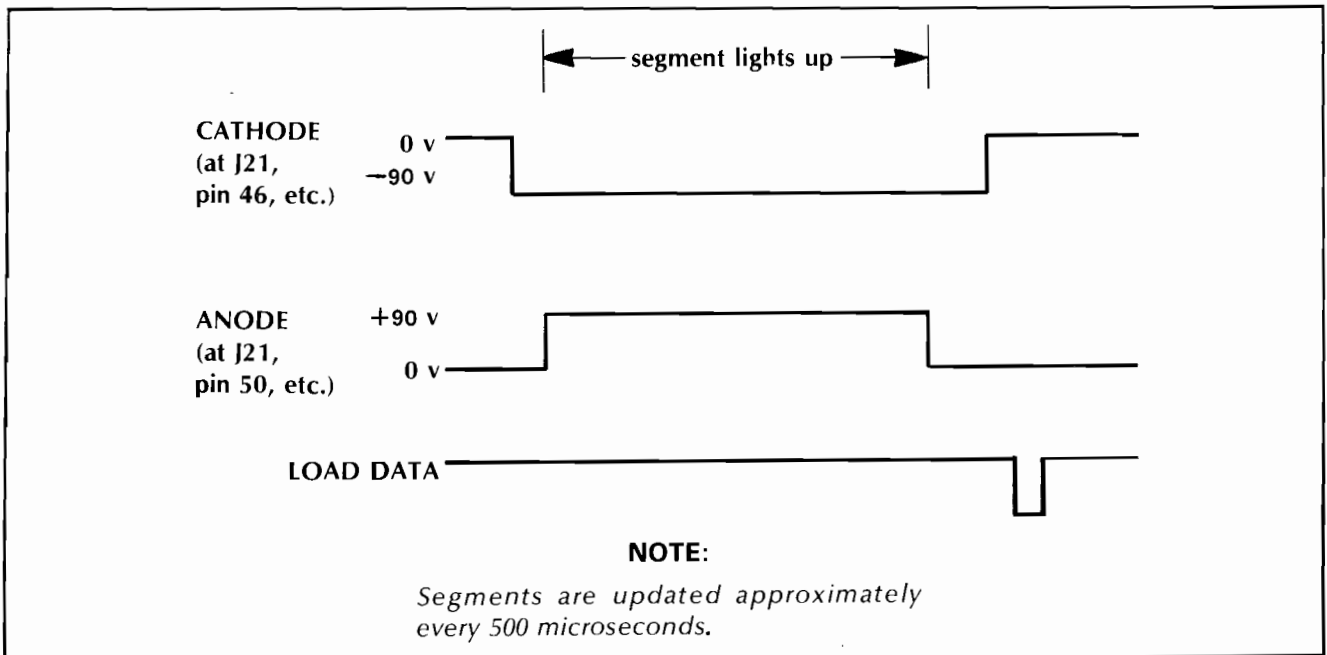
Figure 34 Waveforms for Gas Discharge Displays
