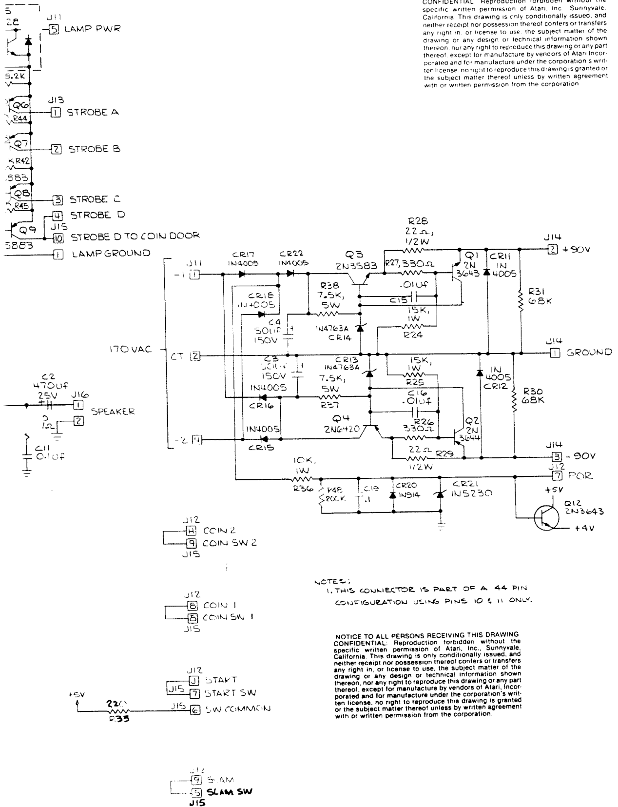
Figure 26 Auxiliary PCB Schematic Diagram 006407-01
