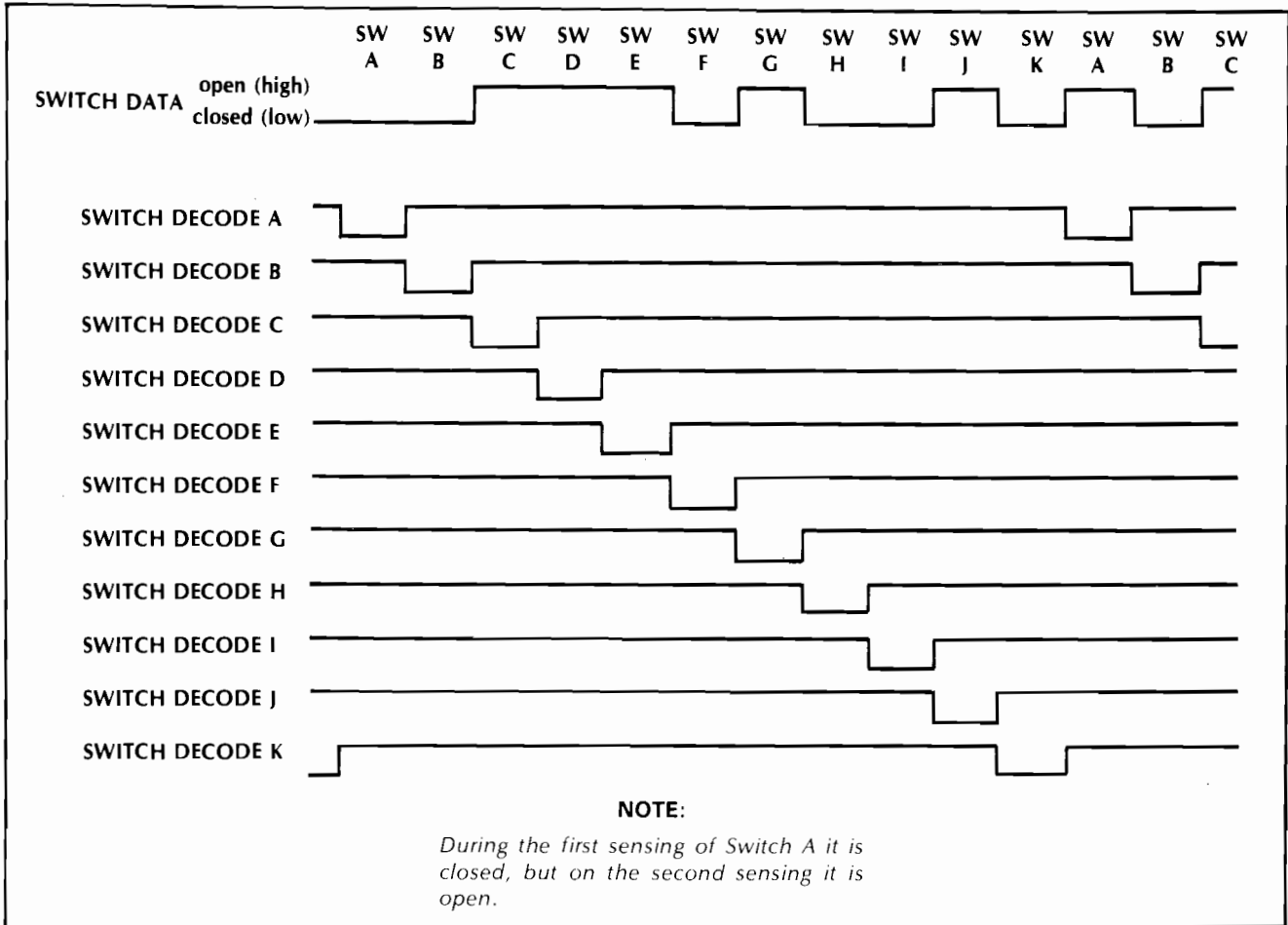
Figure 33 Simplified Diagram of Switch Sensing Circuit Waveforms
