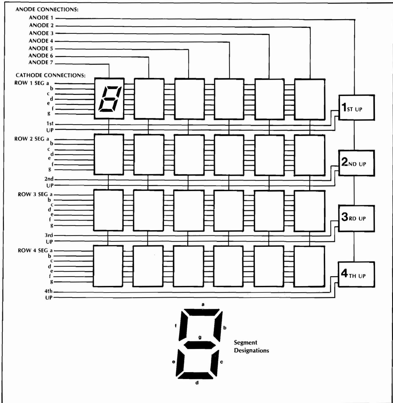
Figure 35 Arrangement of Connections to Score Panel
