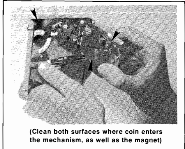
Figure 11 Surfaces to Clean Inside the Coin Mechanism
