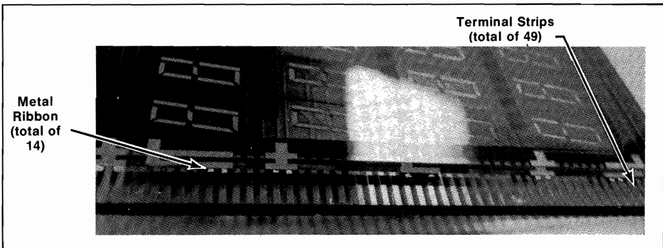
Figure 18 Score Panel Terminals
